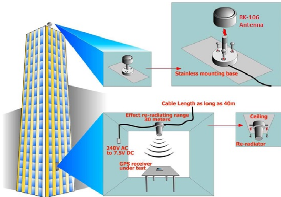
RK-106 Interconnection Diagram
